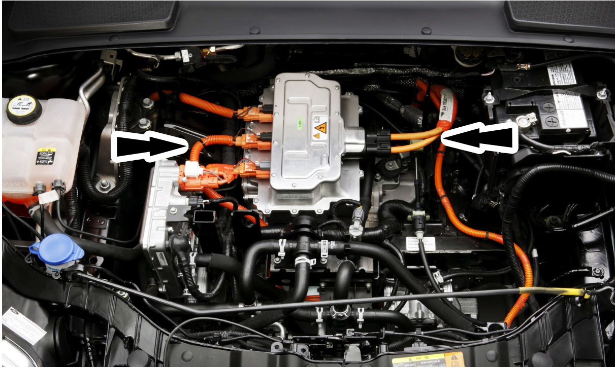
Orange high-voltage cabling from the high-voltage battery packs
